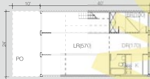
1595 SQF / 3 BEDROOMS / 2 1/2 BATHROOMS / DOUBLE HEIGHT LIVING ROOM / PORCH/ TERRACE
