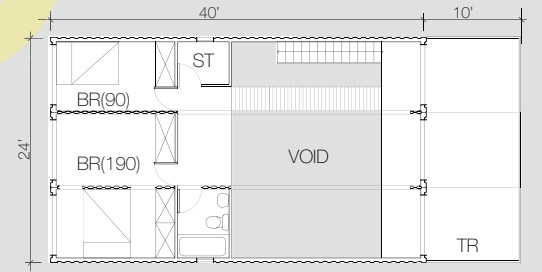
1280 SQF / 2 BEDROOMS / 1 1/2 BATHROOMS / STORAGE-LAUNDRY or ADDITIONAL FULL BATHROOM / OPEN LIVING ROOM / PORCH/ TERRACE
