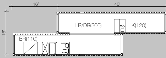
640 SQF / 1 BEDROOM / 1 BATHROOM / OPEN LIVING ROOM
