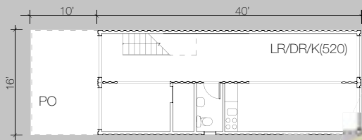
1280 SQF / 2 BEDROOMS / 1 1/2 BATHROOMS / STORAGE-LAUNDRY or ADDITIONAL FULL BATHROOM / OPEN LIVING ROOM / PORCH/ TERRACE
